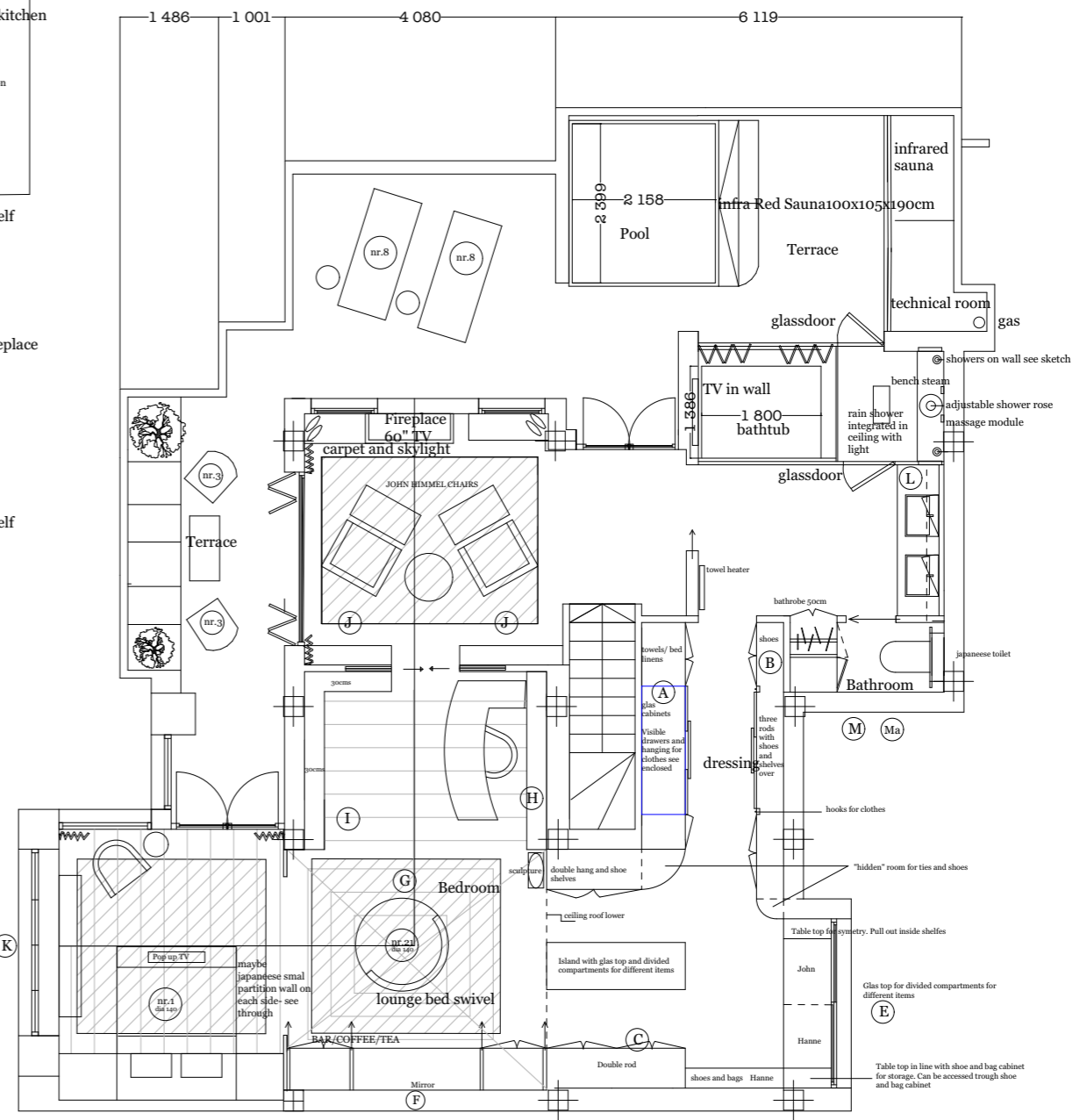
second floor plan 1:100
